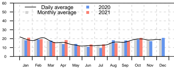
Data period: 16-Aug-2017 to 15-Oct-2021 Daily windrun (3 – 25 m/s) km/day
